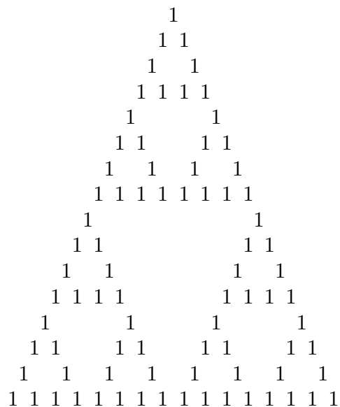
Figure 1: Pascal's triangle mod 2.
